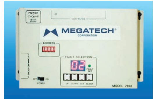
MEG701514 Fault Insertion Box (Required)
